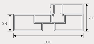
ALEXA 100SG - Timber Door
