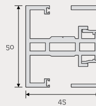
Door Rebate Profile with over panel clip
