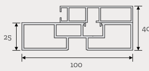
ALEXA 100SG - Glass Door
