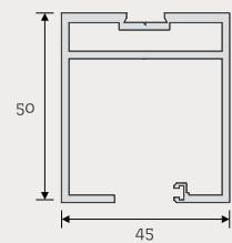
End Profile
